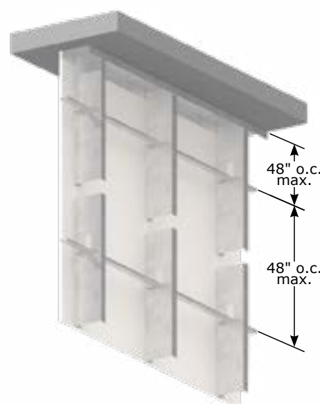
Non-Composite: Braced at 48" o.c. Gypsum board placed on only one side
