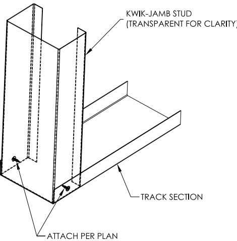
Stud to Track Connection
