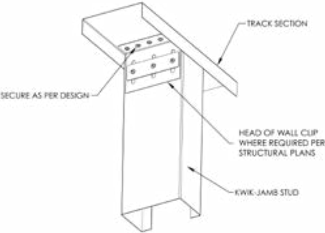
Head of Wall Connection
